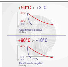
Chilling cycle
