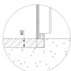
Scheme for floor recessed installation
