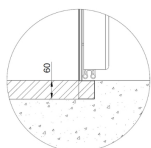
Scheme for floor recessed installation
