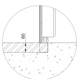
Scheme for floor recessed installation
